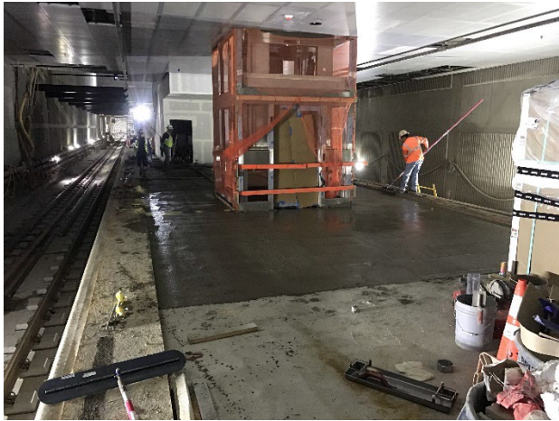
BDS Topping Slab at Platform Level
