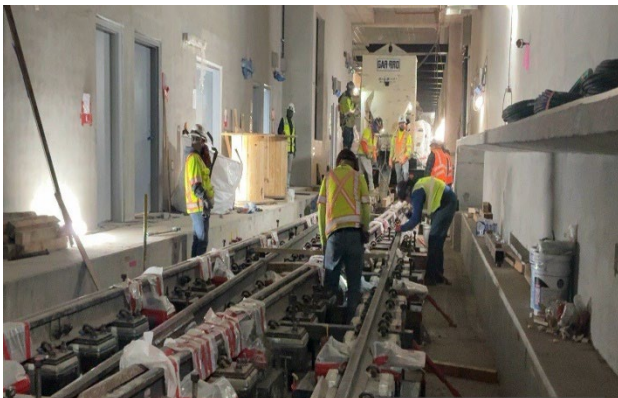
CCS DXO Sleeper Concrete Placement BR
