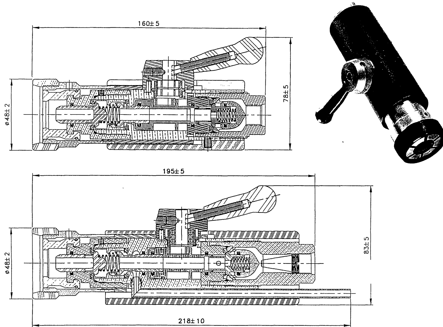
Figure 2.3.A Example of Type 1 Nozzle From Two Manufacturers
