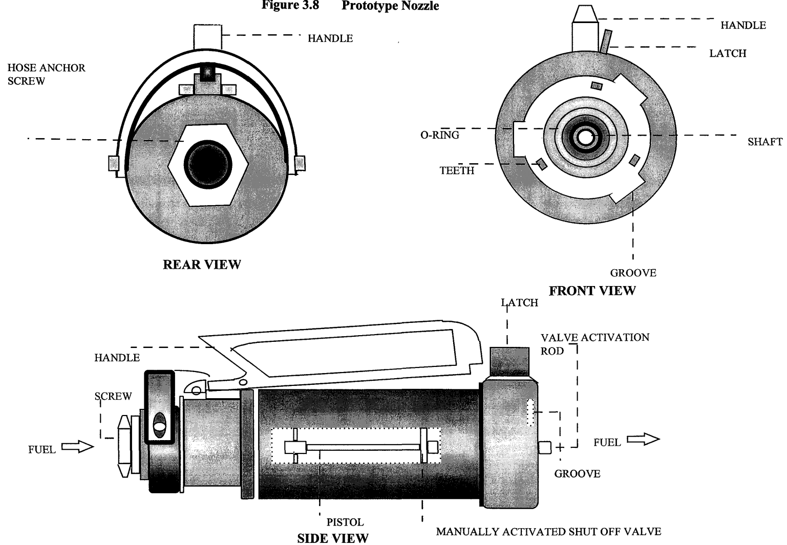
Figure 3.8 Prototype Nozzle
