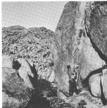
Survey Party Chief Walter Butcher, a District 11 employee, setting slope stakes in rock.
