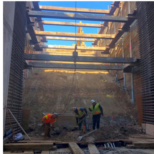
Westwood/UCLA Station: Main Entrance Sloped Portal Excavation
