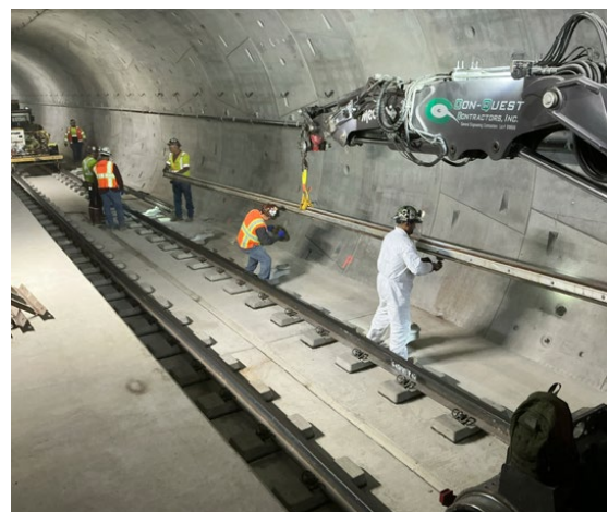
Tunnels/Track: Contact Rail Installation on Insulators in the BL Tunnel Reach 6
