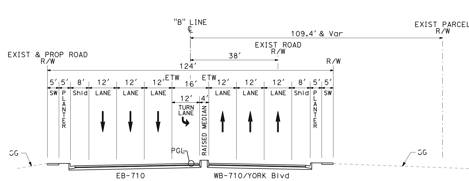
SECTION D-D SR-710/YORK BLVD NTS
