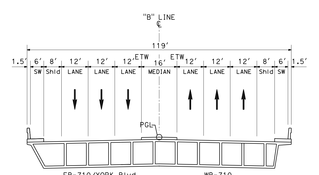
SECTION C-C SR-710/YORK BLVD NTS
