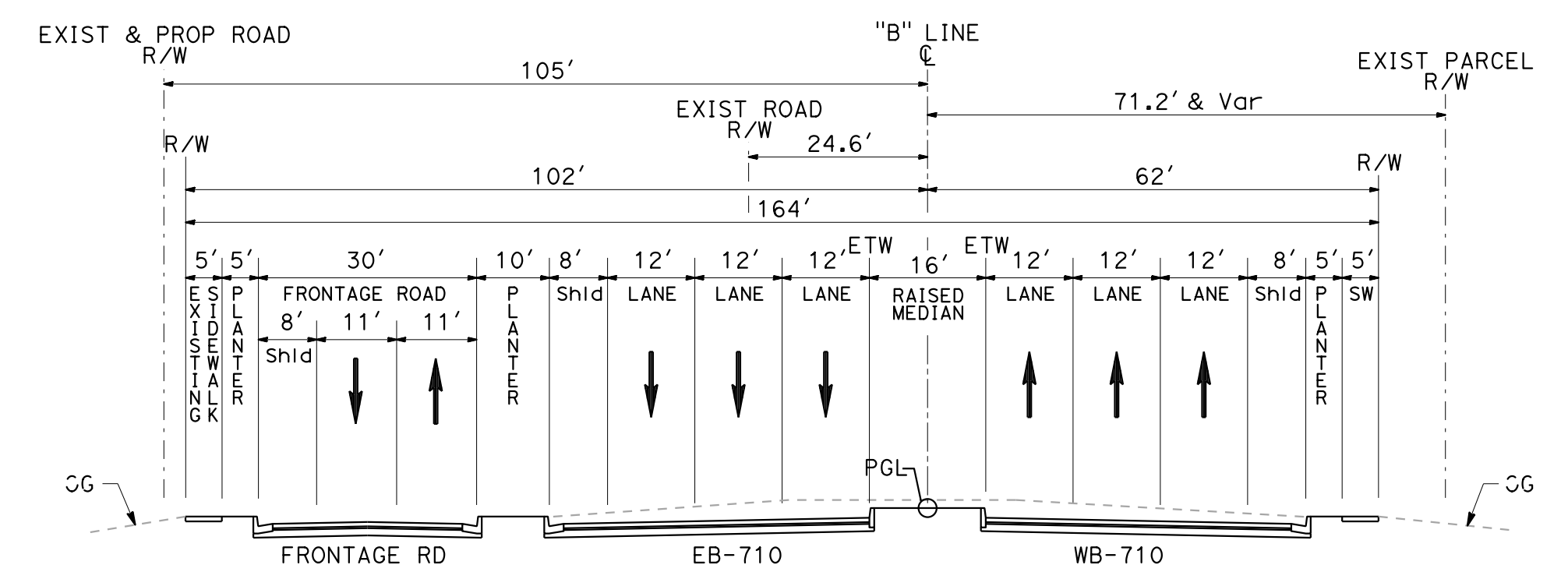
SECTION B-B SR-710/MONTERREY RD NTS
