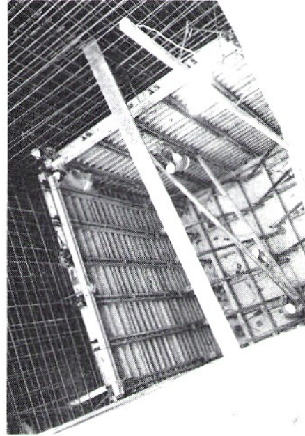
FORMING VERTICAL WALLS AT SOUTH BLAST RELIEF SHAFT
