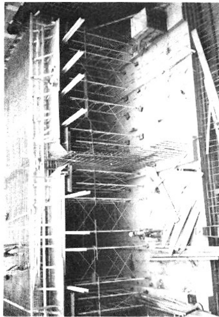
FORM SUPPORT SYSTEM FOR BOX STRUCTURE ROOF SLAB
