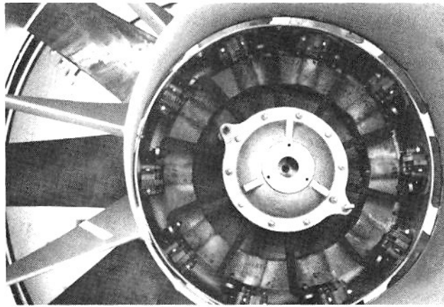
VARIABLE PITCH MECHANISM FOR UNDERPLATFORM FAN/MOTOR
