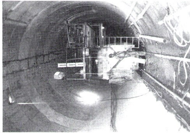
PLATFORM MOUNTED ON RAILCAR FOR SAWCUTTING CONCRETE SEGMENTS PRIOR TO CROSS PASSAGE EXCAVATION IN AL TUNNEL
