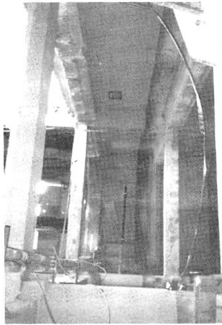
DEMOLITION OF ROOSEVELT BUILDING 1ST FLOOR AND BASEMENT SLABS
