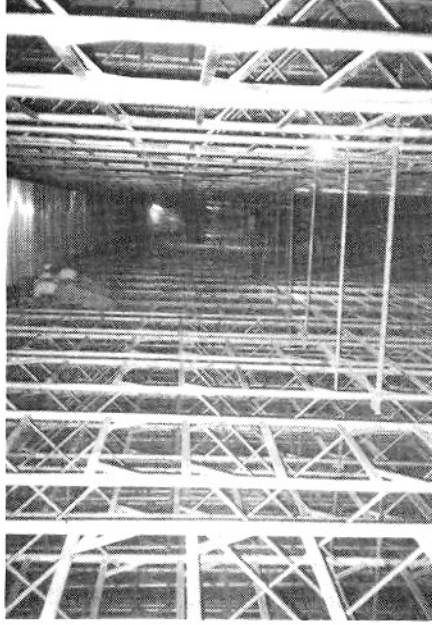
LEVELING SHORING FOR ANCILLARY SLAB POUR IN CIVIC CENTER STATION
