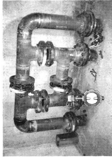
WET STAND PIPE VALVE ASSEMBLY IN SUMP ROOM
