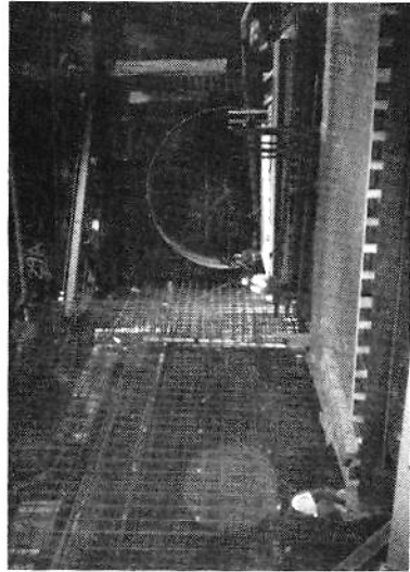
PREPARING THE EAST WALL FORMS AT SECTIONS 15/16. ALSO VISIBLE ARE THE TUNNEL RINGS AT THE SOUTH END OF THE STATION
