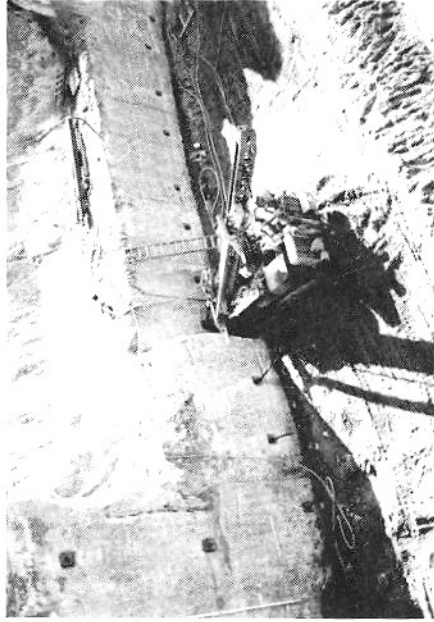
INSTALLATION OF TIEBACK ANCHOR TENDONS THRU SLURRY WALLS
