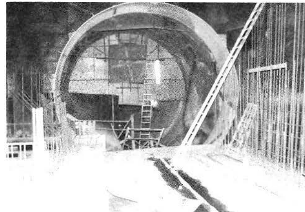
SOUTHEAST AIR TUNNEL; TUNNEL RING IN PLACE
