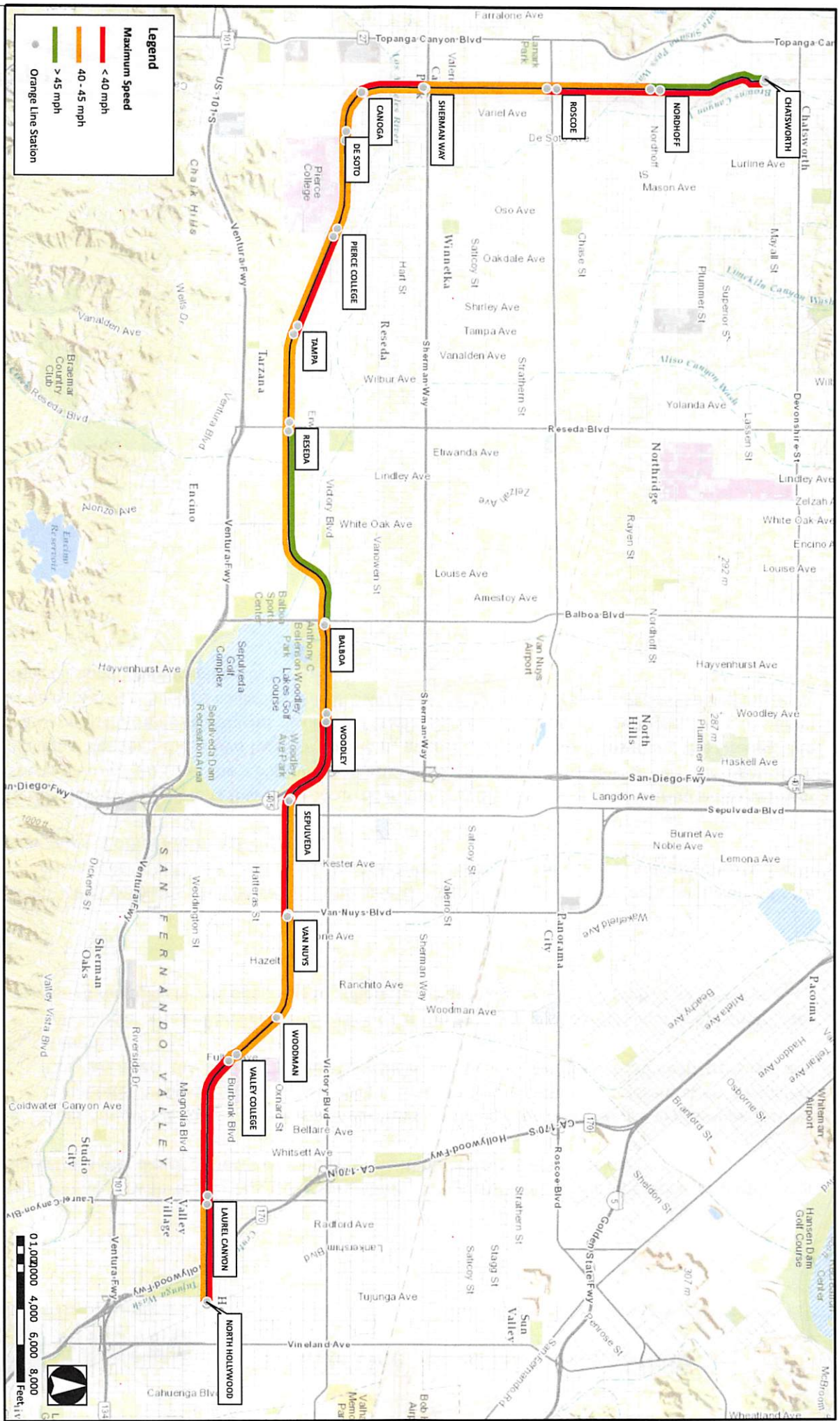
Figure 6 MOL Maximum Speed
