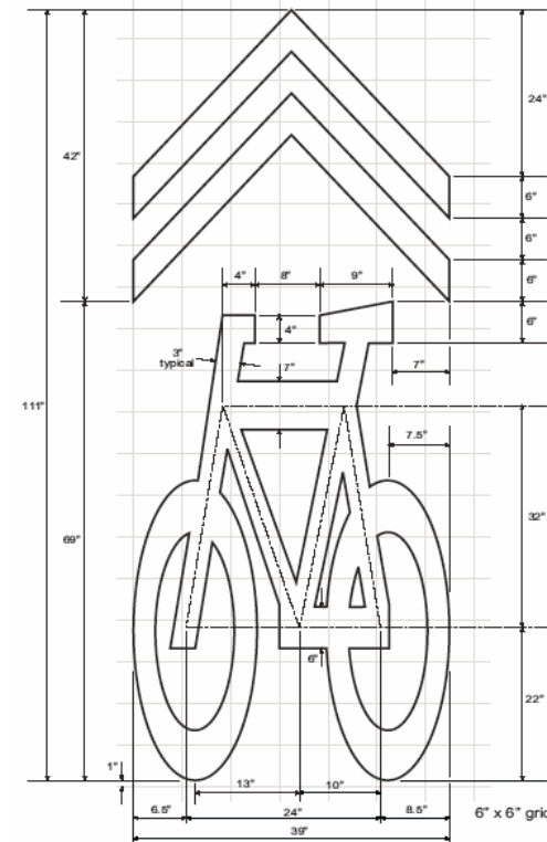
NO SCALE Shared Lane Marking
