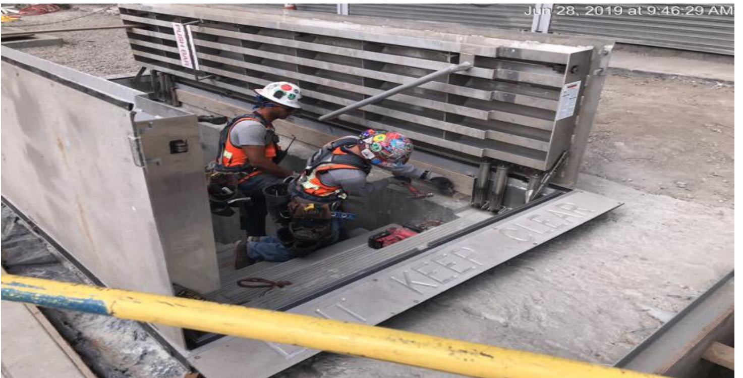
EXPOSITION/CRENSHAW STATION – Installation of plywood form for Emergency Exit #2 south at the roof level.
