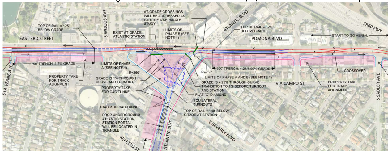
Figure 3-8. Combined Alternative Wye Junction Potential Land Acquisition
