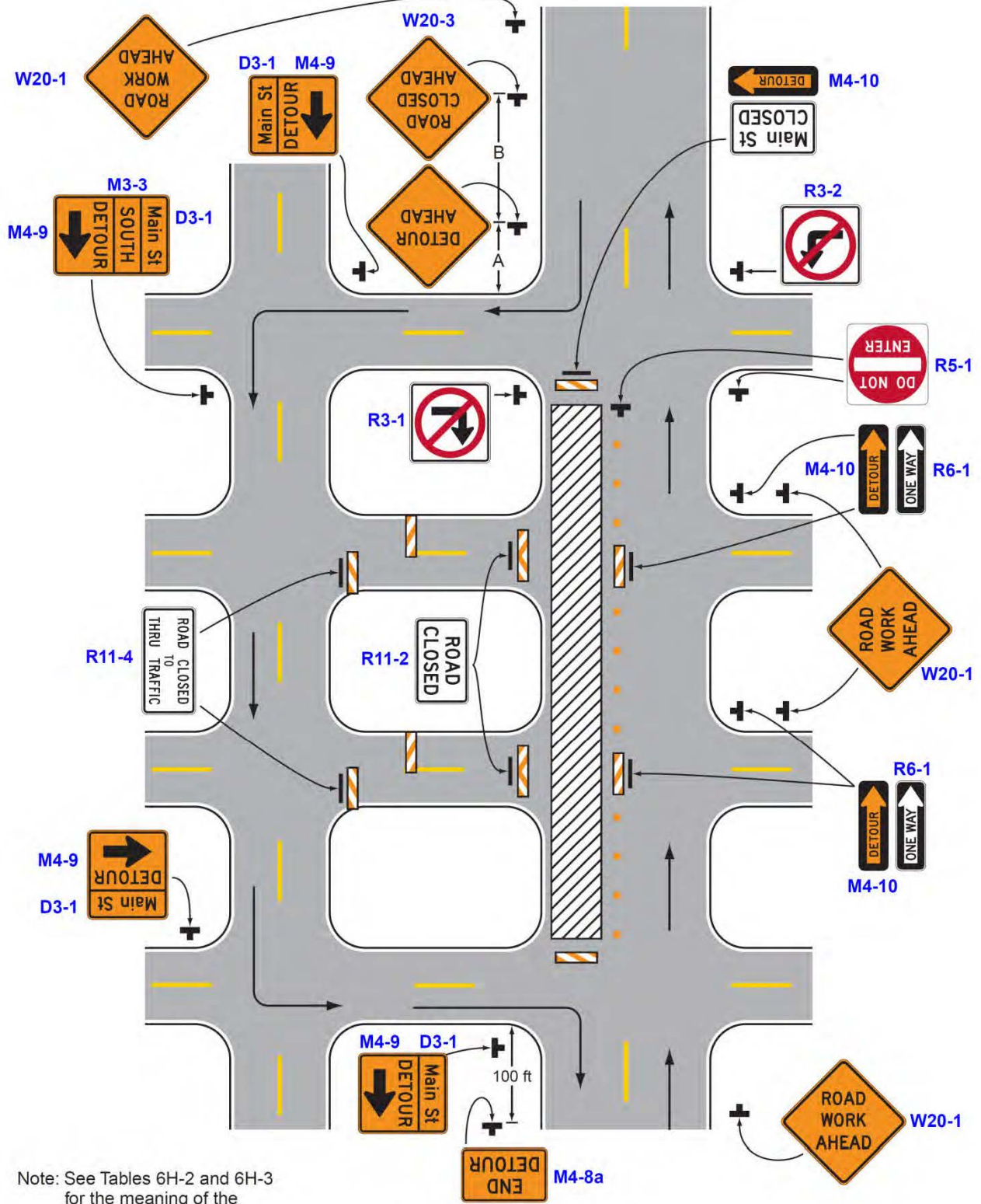
Typical Application 19
