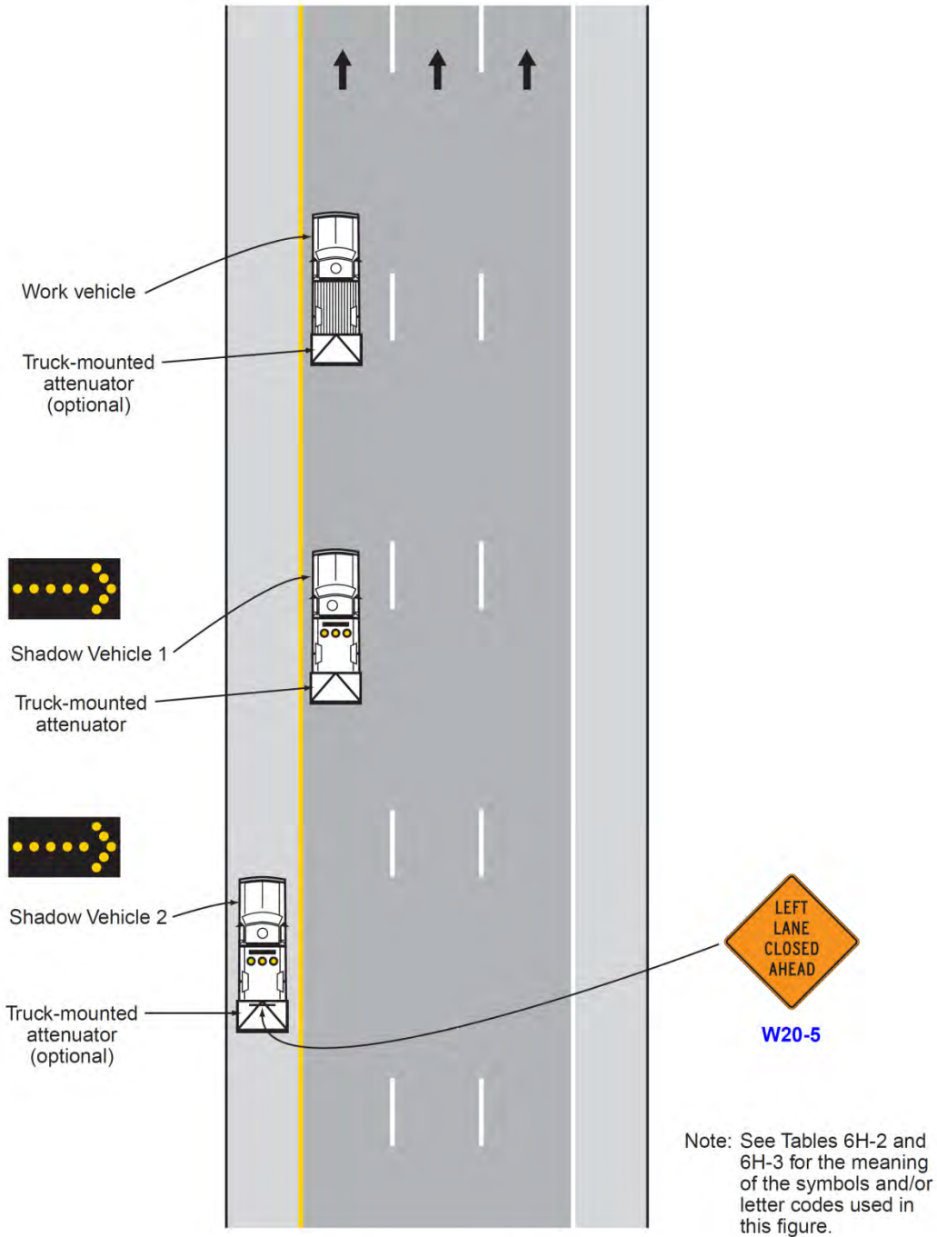
Typical Application 35
