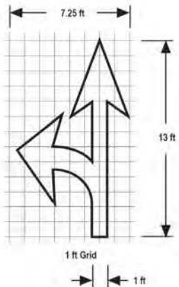
TYPE VII (L) ARROW (FOR TYPE (R) ARROW, USE MIRROR IMAGE)
