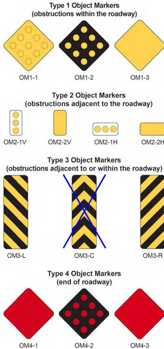
Figure 2C-13. Object Markers
