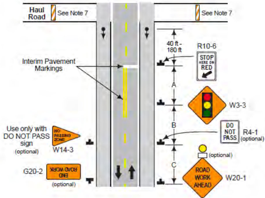
Figure 6H-14 (CA). Haul Road Crossing (TA-14)
