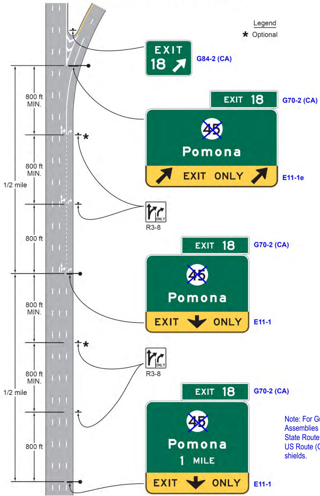
Figure 2E-11. Example of Signing for a Two-Lane Intermediate or Minor Interchange Exit with an Option Lane and a Dropped Lane
