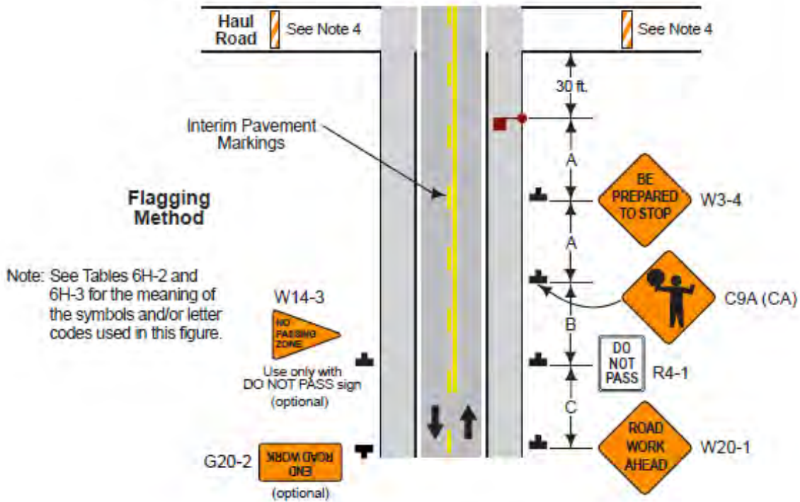
Typical Application 14
