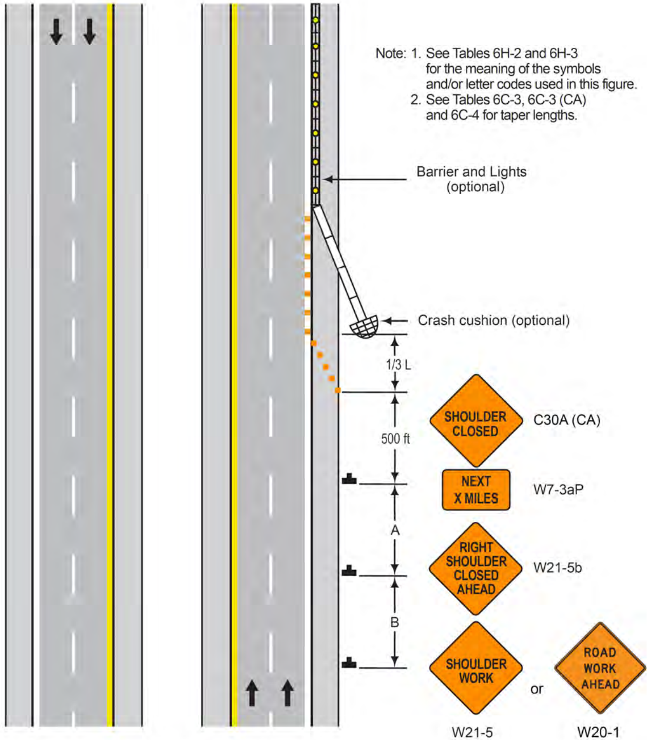
Typical Application 5
