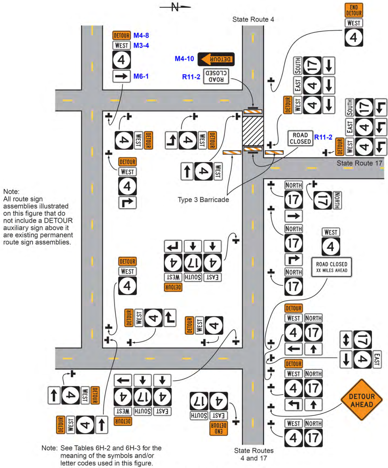
Typical Application 9
