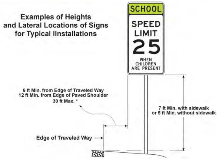
Figure 7B-1(CA). School Area Signs (Sheet 2 of 2)
