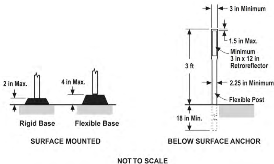
Figure 3H-101 (CA). Example of Channelizers
