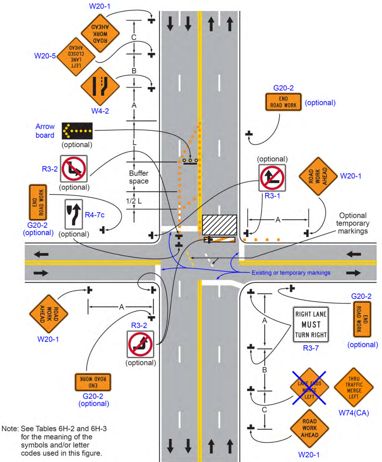
Typical Application 24
