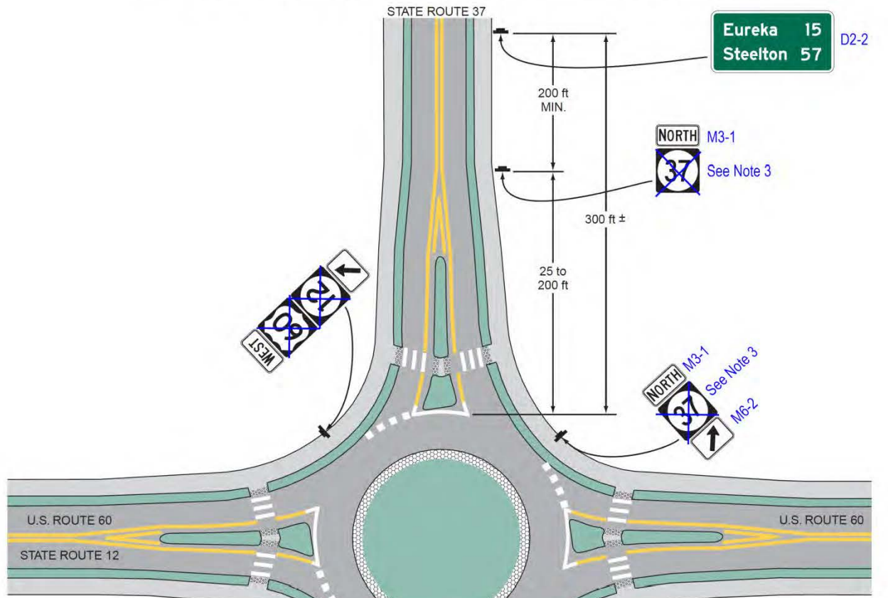
Figure 2D-9. Examples of Guide Signs for Roundabouts (Sheet 2 of 2)
