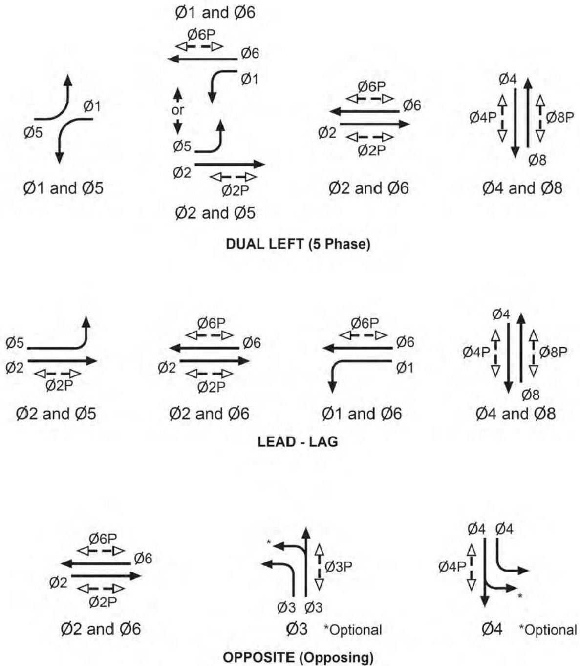
Figure 4D-101 (CA). Left-Turn Phasing Methods(Phase Diagrams)
