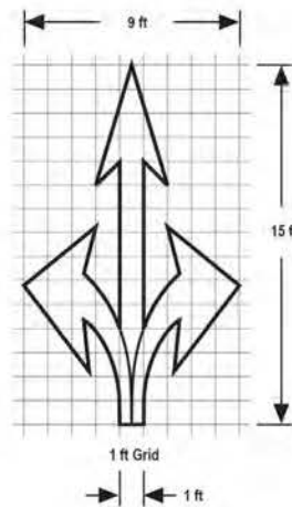
TYPE VIII ARROW
