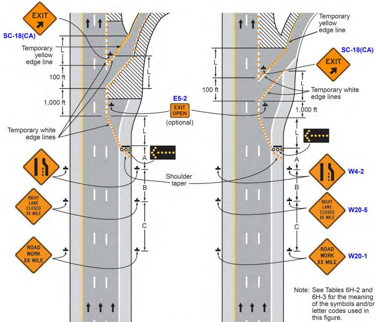
Typical Application 42
