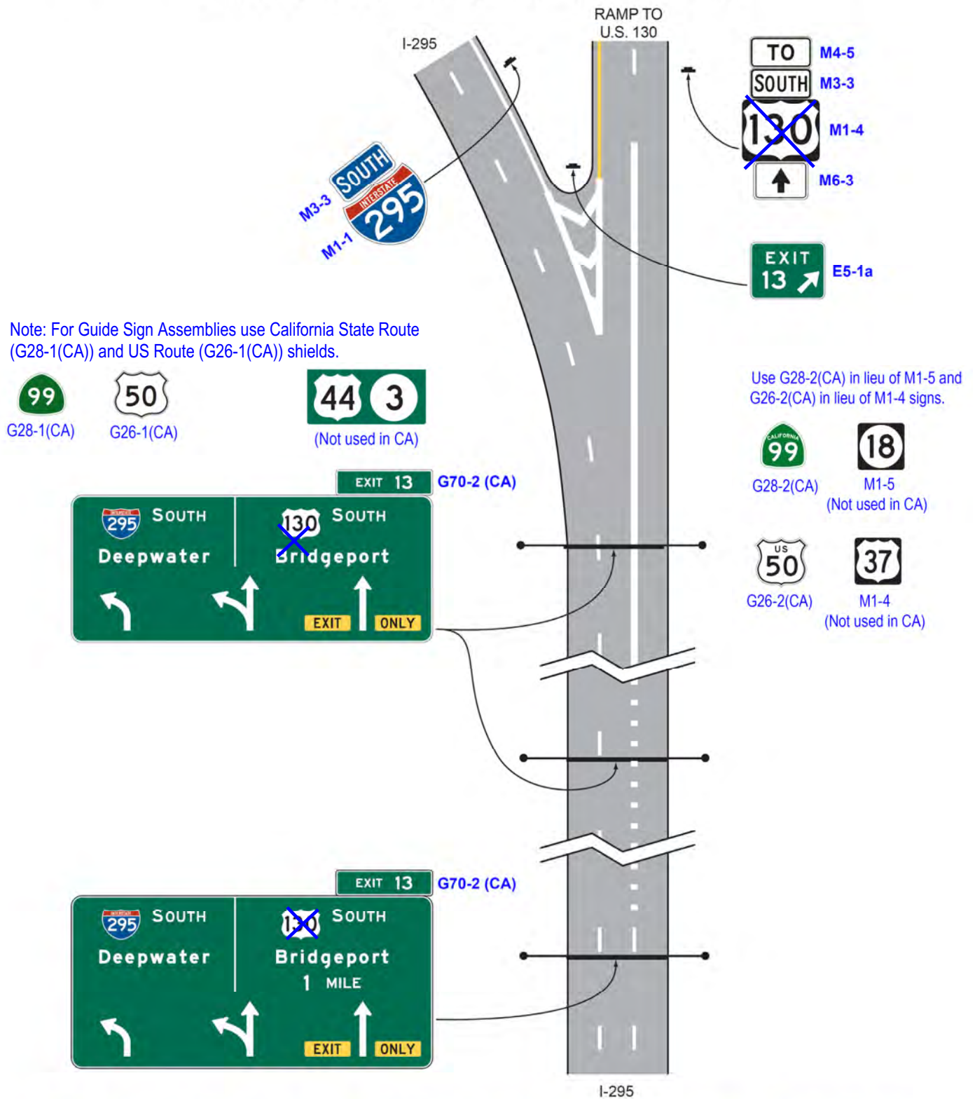
Figure 2E-5. Overhead Arrow-per-Lane Guide Signs for a Two-Lane Exit to the Right with an Option Lane (Through Lanes Curve to the Left)
