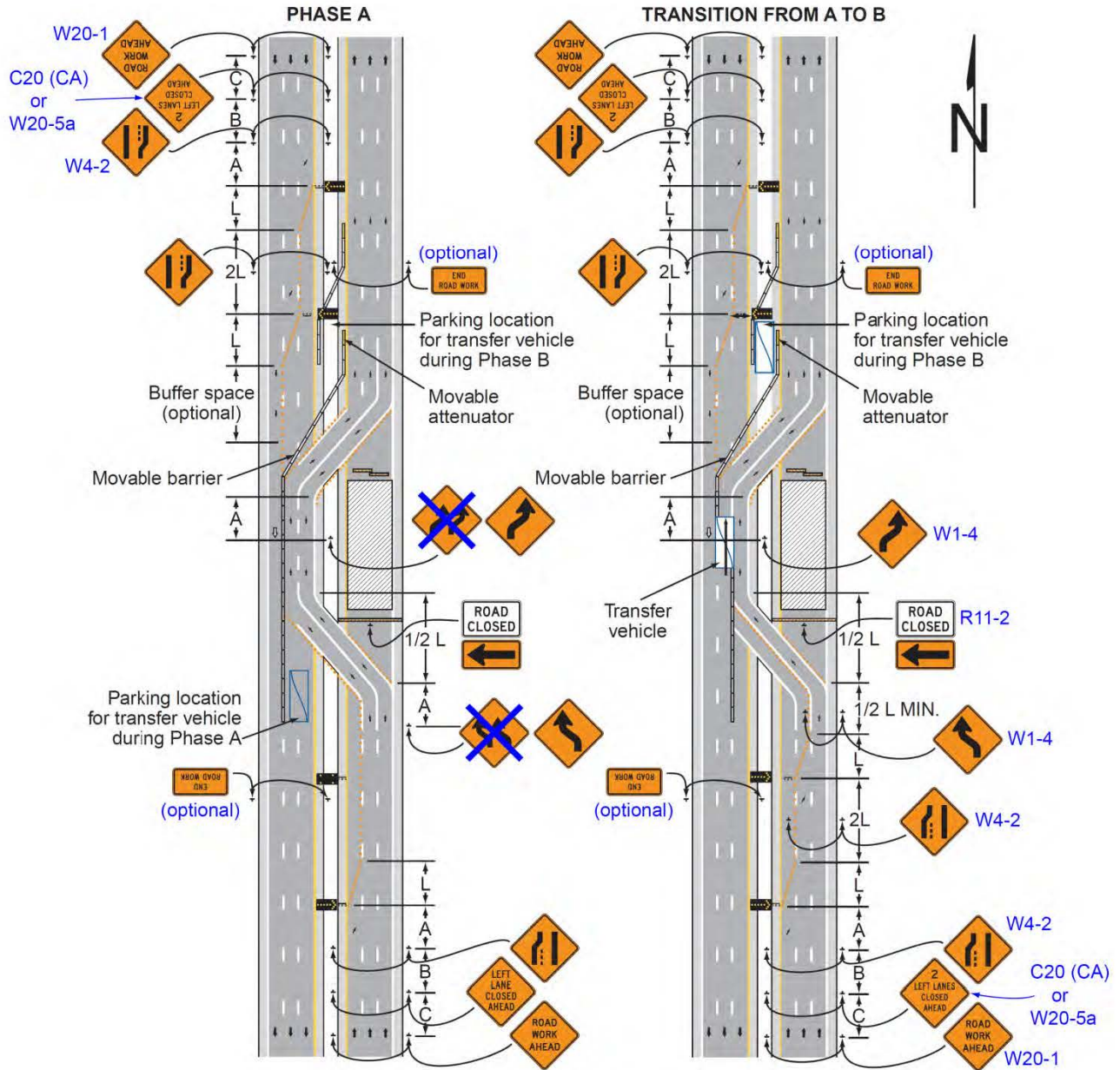
Typical Application 45
