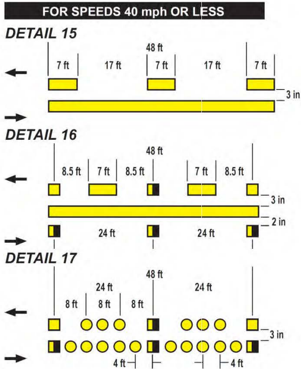
Figure 3A-103 (CA). No Passing Zones - One Direction
