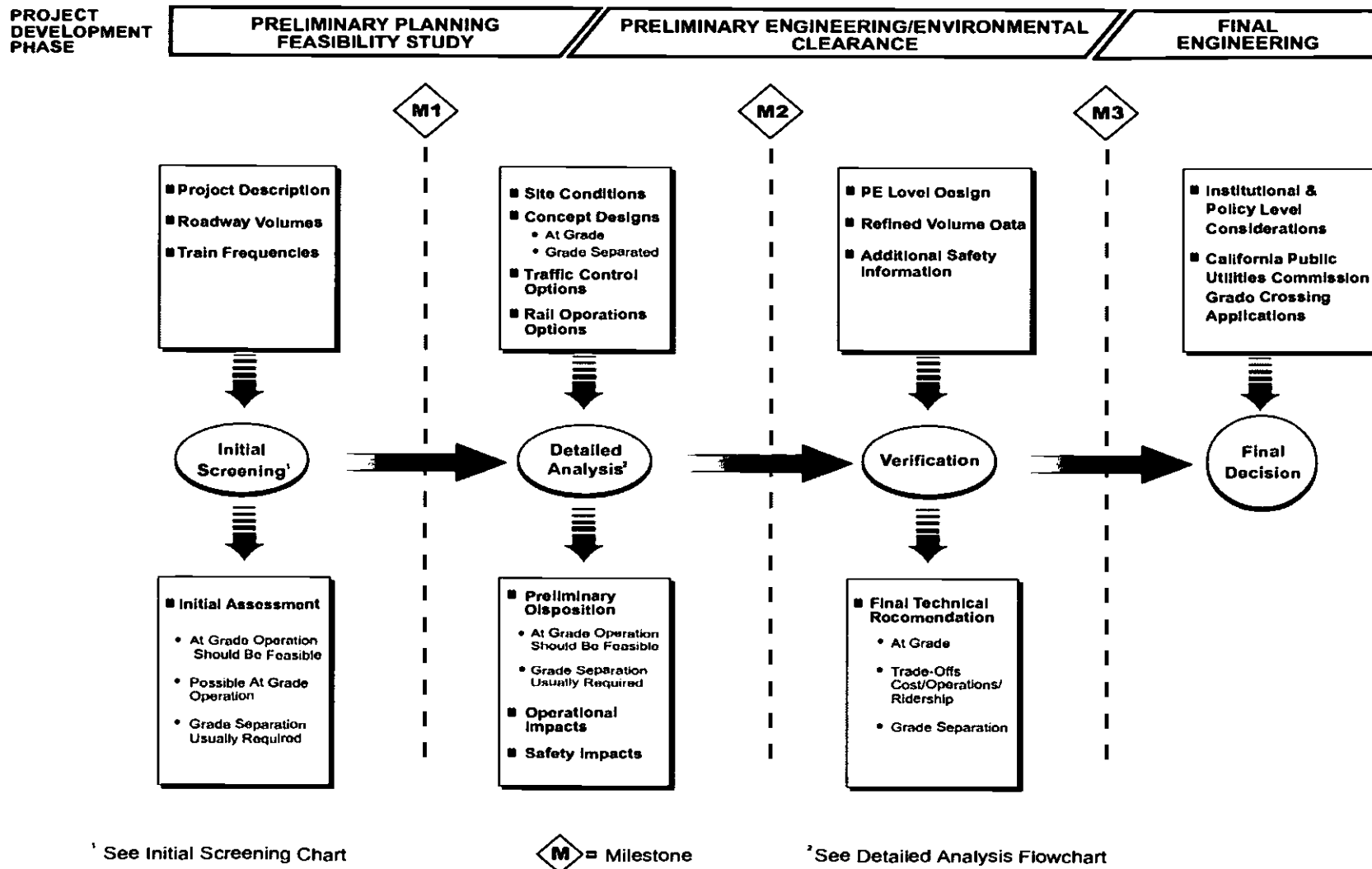
Figure 1 – Light Rail Roadway Crossing Review Process
