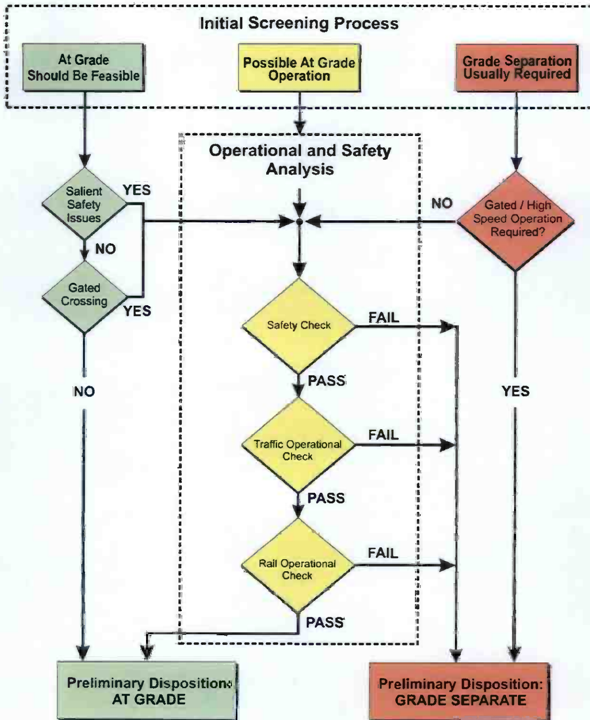
Figure 2 – Evaluation Flowchart
