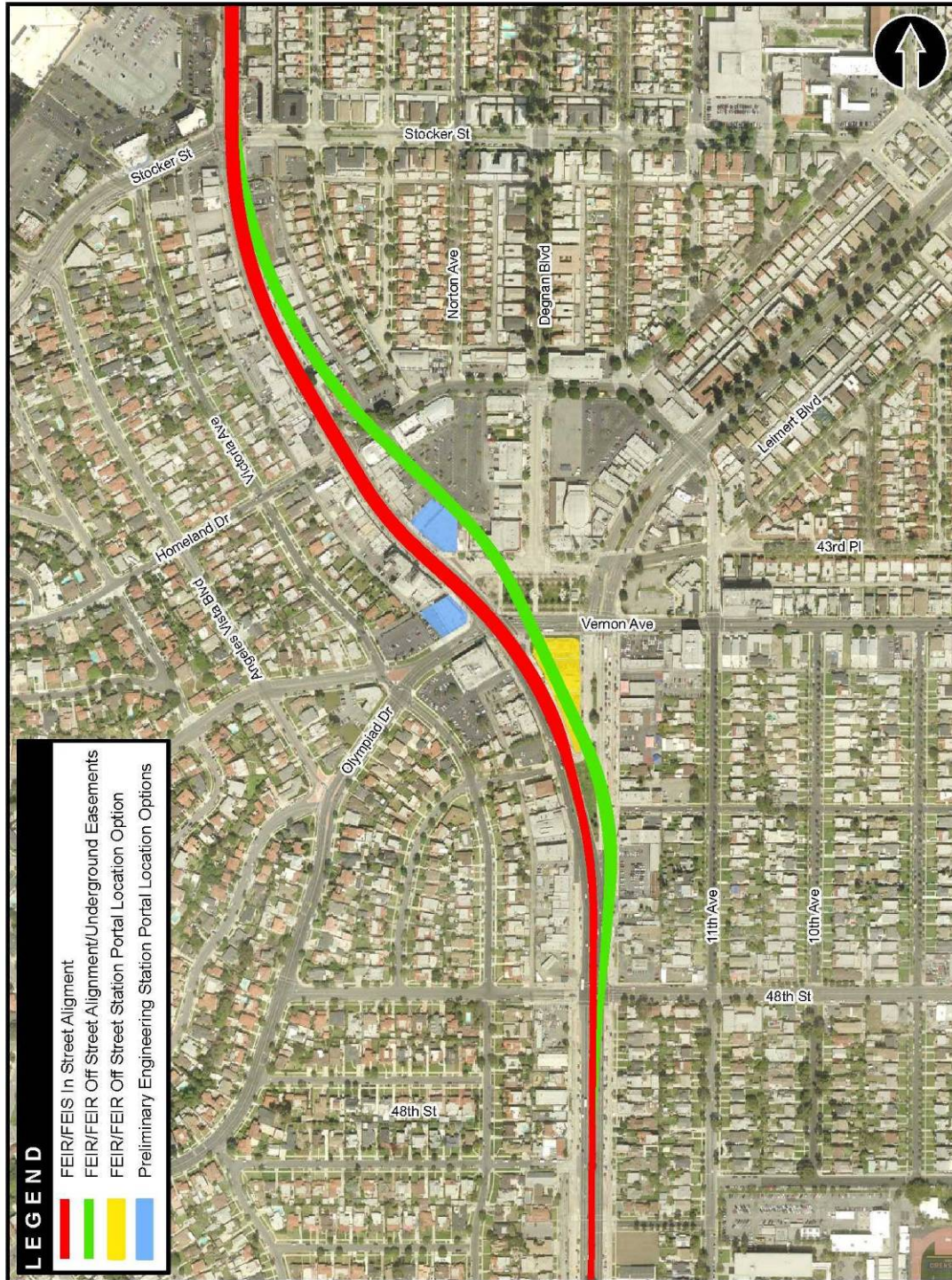
Vernon exhibit – change from FEIS/FEIR is alternate In-Street Vernon Station location.
