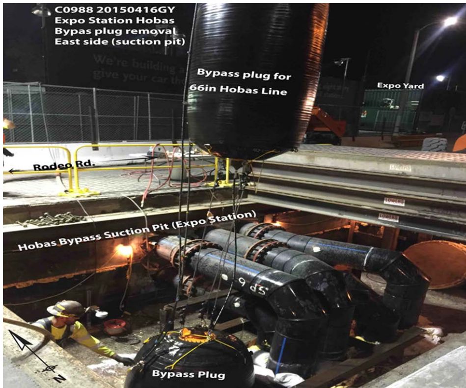
Dual Plug Removal Allowing Flow to Start in. New 66" Hobas Sanitary Sewer at Expo Station.
