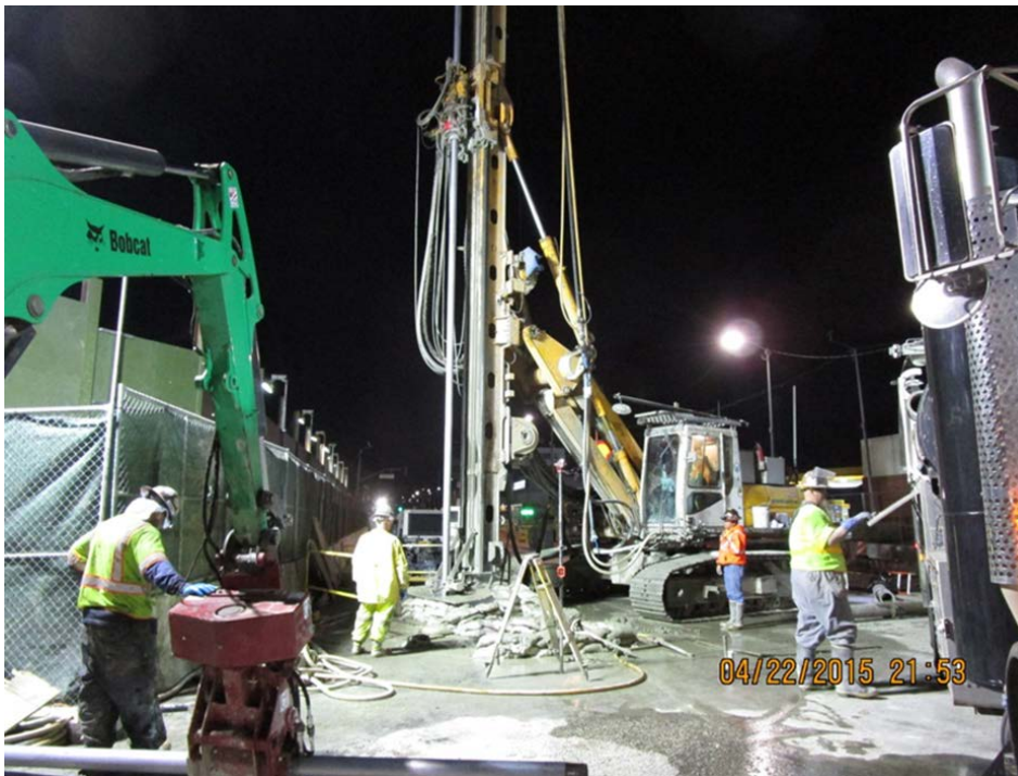
Jet Grouting SOE North Headwall, Expo Station.
