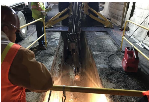
DWP Power Relocation on Flower Street
