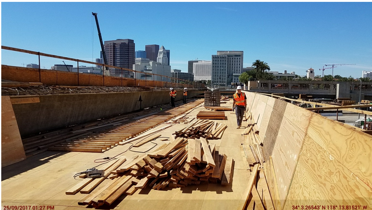
Form girders on falsework Frame 3 LT.
