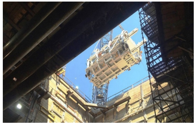
Lowering TBM Equipment at Wilshire/La Brea Station
