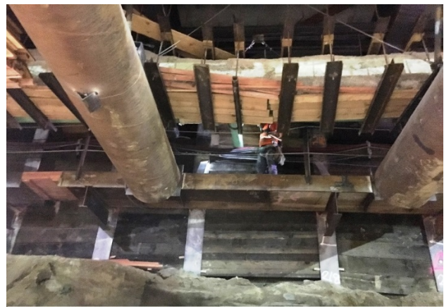
AT&T Ductbank at Wilshire/La Cienega Station
