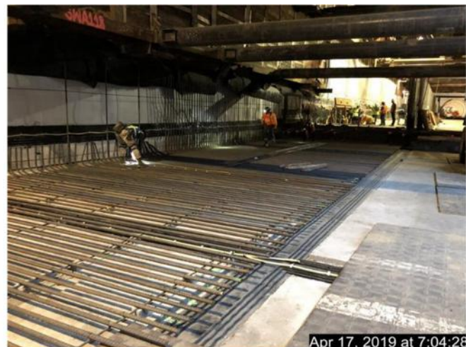
Bottom mat rebar installation; Areas 7 and 8 at north Flower St
