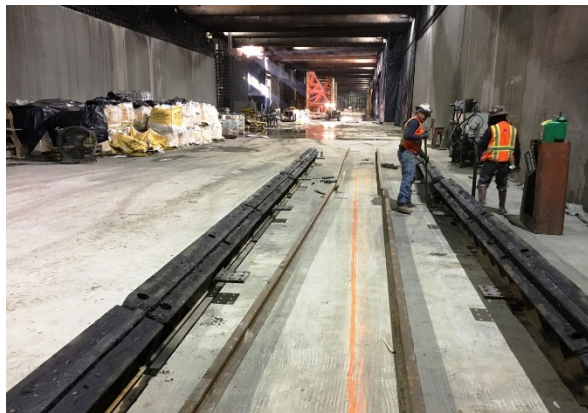
Temporary Rail Installation at Wilshire/Fairfax Station
