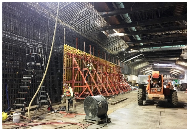
2 nd Lift Exterior Wall Forms at Wilshire/La Brea Station
