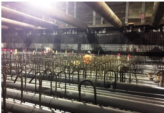
Invert Rebar Installation at Wilshire/La Cienega Station
