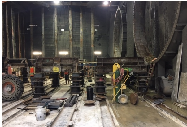
TBM Cradle Assembly at Wilshire/Western
