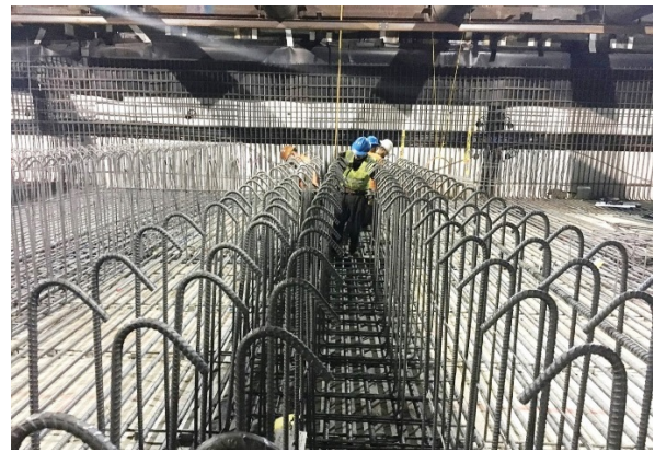
Wilshire/Fairfax Station Invert Rebar
