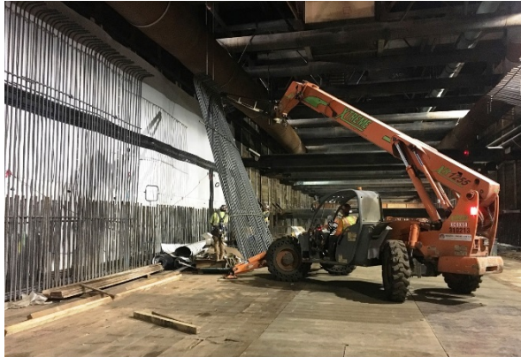
Concourse Wall Rebar at Wilshire/La Brea Station
