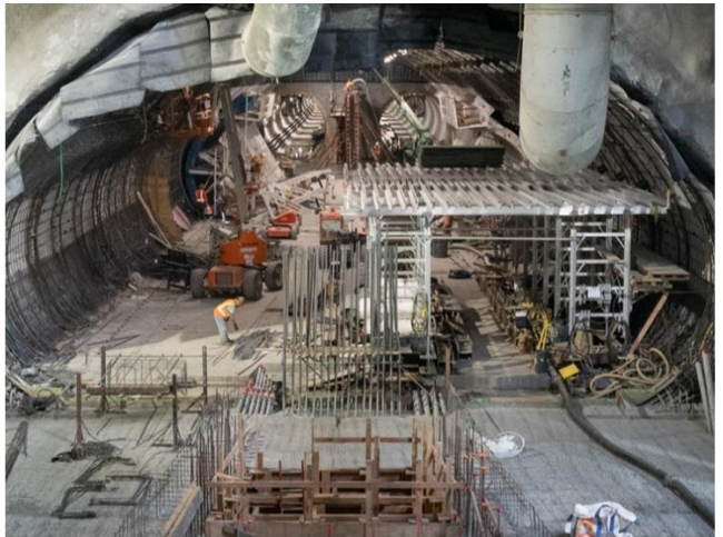
SEM Cavern overview from west
