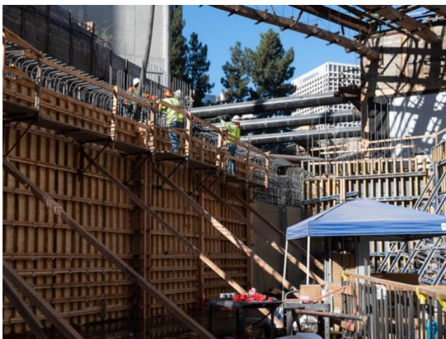
Setting wall forms at Concourse Level of Grand Av Arts/Bunker Hill Station
