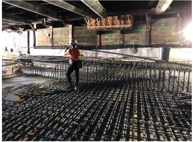
Bottom mat rebar installation for track roof slab at the Wye
