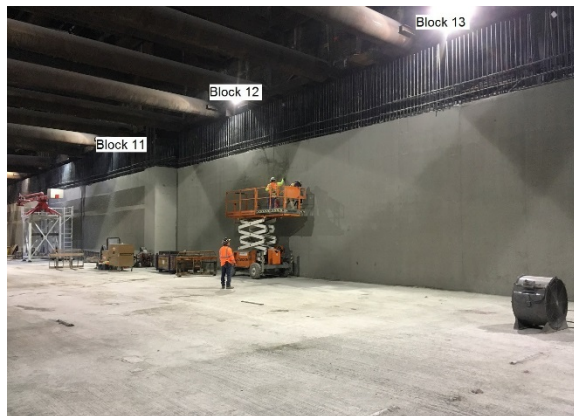
Lift 1 Exterior Walls at Wilshire/Fairfax Station
