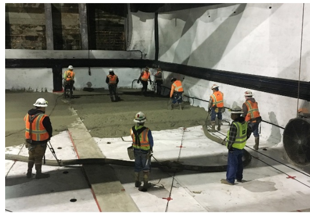
Concrete Placement at Wilshire/La Cienega Station
