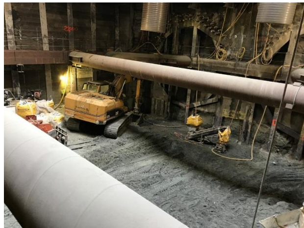
TBM Launch Box Excavation in Century City
