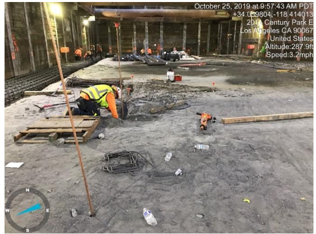
TBM Launch Box Excavation in Century City
