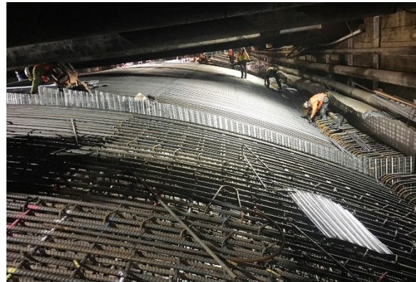
Roof Rebar Installation at Wilshire/La Brea Station
