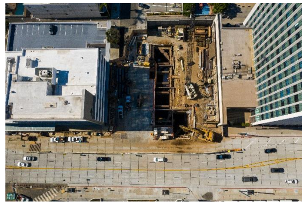
Wilshire/Rodeo Station Entrance Excavation Activities
