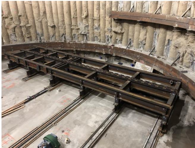
Superstructure at Base of Excavated Tail Track Exit Shaft
