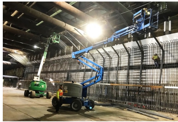
2 nd Lift Rebar Installation at Wilshire/La Cienega Station
