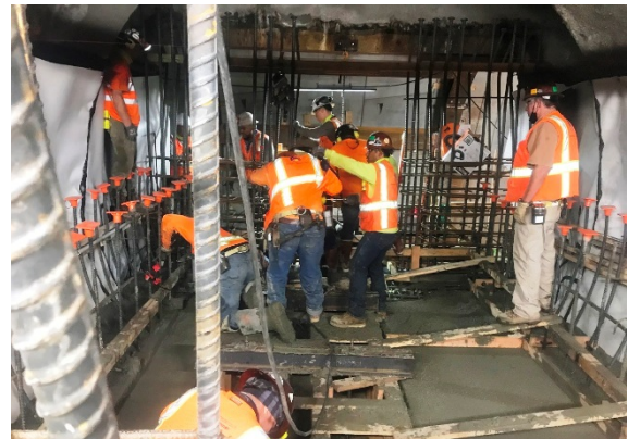
Cross Passage #11 Invert Concrete Placement
