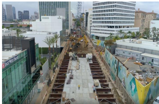
Wilshire/Rodeo Station Pile Installation and Decking During the Temporary Full Street Closure
