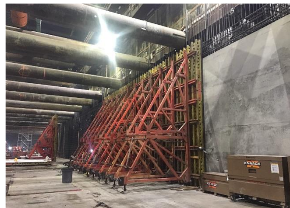
Concrete Placement for First Level Station Walls
