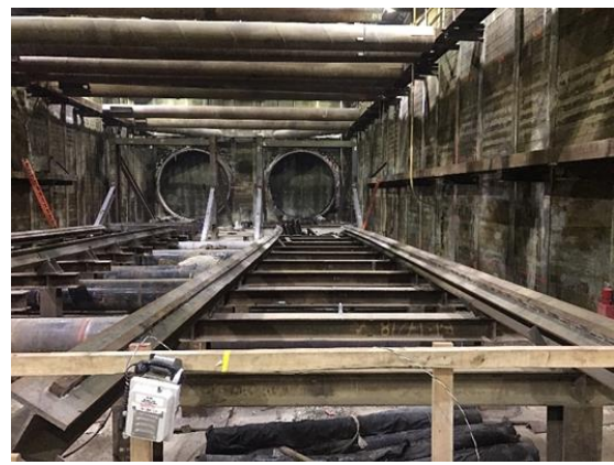
TBM Cradle Frame, TBM Break-Out (East)
