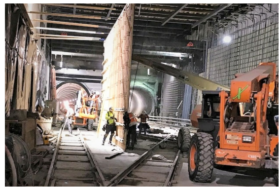
Interior Wall Formwork at Wilshire/La Cienega Station
