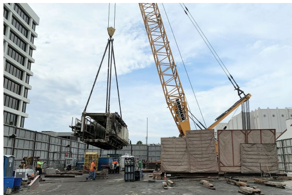
TBM Gantry Removal from the Gale Yard
