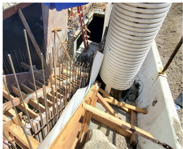
Installation of rebar and form at Emergency Exit at Historic Broadway Station
