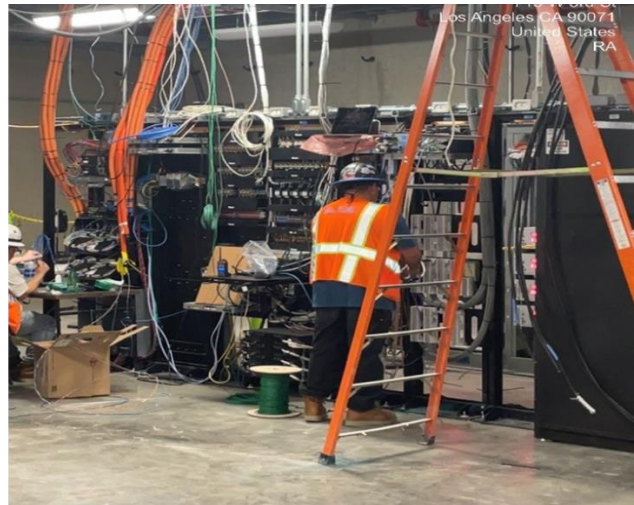
TC&C Room at Grand Av Arts/Bunker Hill Station
