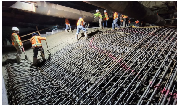
Roof Concrete Placement at Wilshire/Fairfax Station
