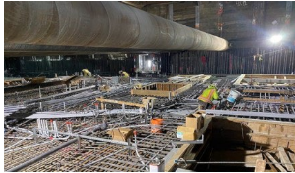
West Concourse Rebar Installation at Wilshire/La Cienega
