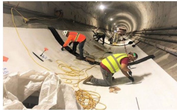
Reach 2 (North) Secondary Gas Liner/Track Invert Membrane
