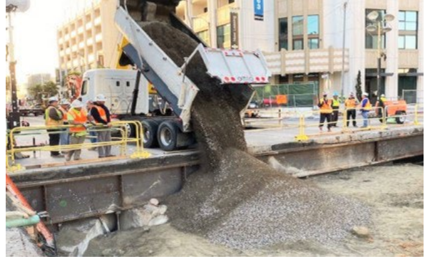
Weekend Decking Removal at Wilshire/La Brea Station
