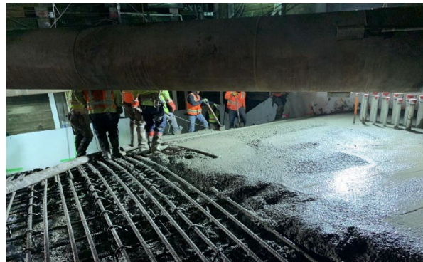
Wilshire/La Cienega Station Box Roof Concrete Placement
