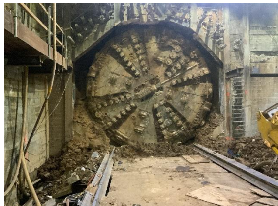
BL TBM Break-In at Wilshire/Rodeo Station
