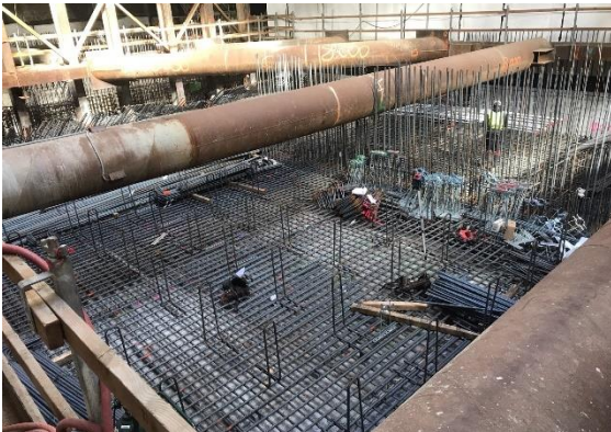
Rebar and Formwork for Wilshire/Rodeo Station Entrance
