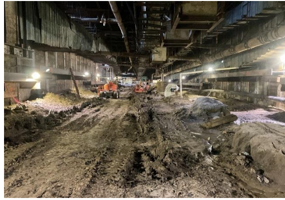
Excavation and Utility Support Activities West of the Launch Box in Century City
