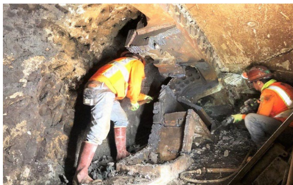
Reach 4 North TBM Cutterhead Removal
