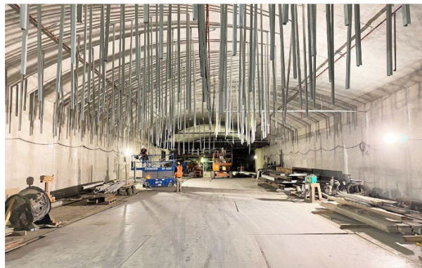
Ceiling Grid Installation at Wilshire/Fairfax Station
