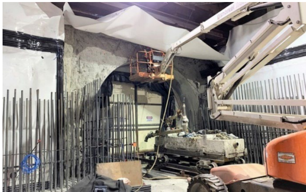
Concrete Wall Construction at Wilshire/Western Shaft
