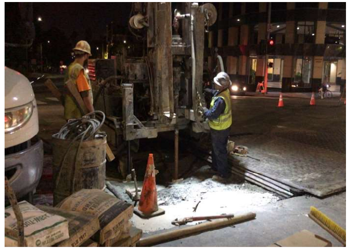
Westwood/UCLA Station SOE Pile Drilling in Wilshire Blvd. Median
