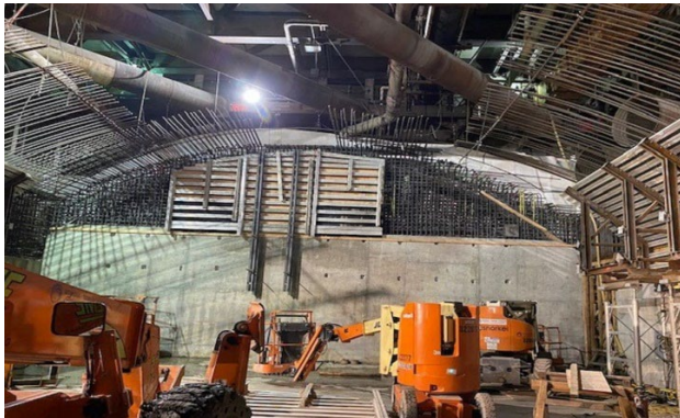
West End Wall Construction at Wilshire/La Cienega Station
