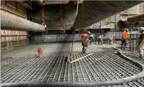
Entrance Structure Concrete Work at Wilshire/La Brea Station
