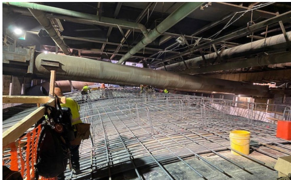
Roof Rebar Placement at Wilshire/La Cienega Station
