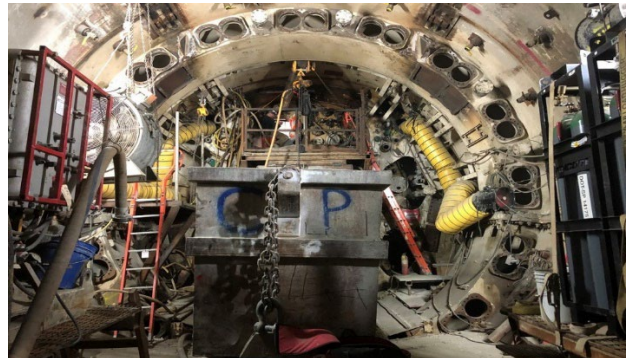
Reach 4 South Tunnel TBM Cutterhead Removal
