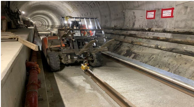
Reach 2 North Tunnel Track Installation
