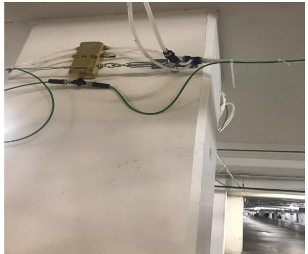
Westfield Mall – Array B Liquid Level Installation
