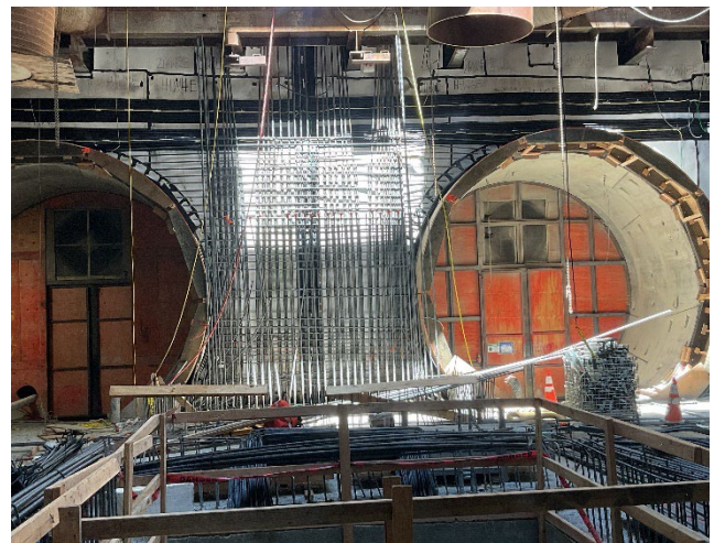
Rebar Installation at CCCS (East Wall)
