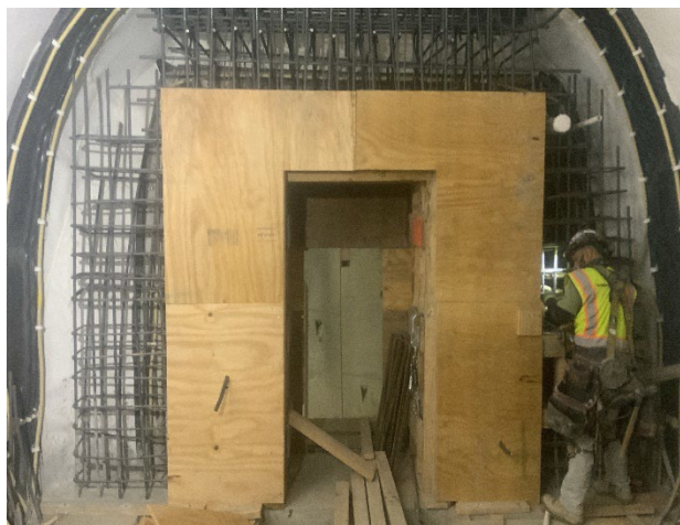
CP-37 Bulkhead Rebar and MEP Install
