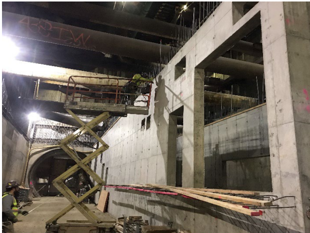
WRS West Hammerhead Interior Walls
