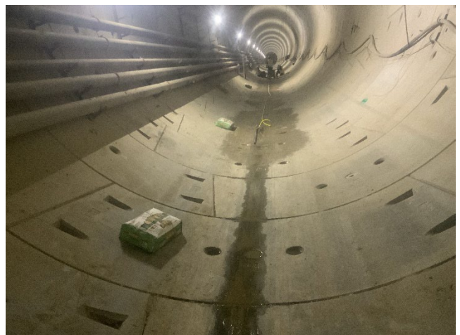
BL Reach 5 Invert Cleaning
