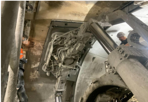
BR Tunnel Cross Passage 43 Ring Installation
