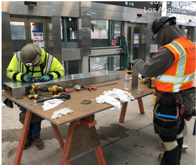
SS cladding installation for elevator towers at Grand Av Arts/Bunker Hill Station Upper Plaza
