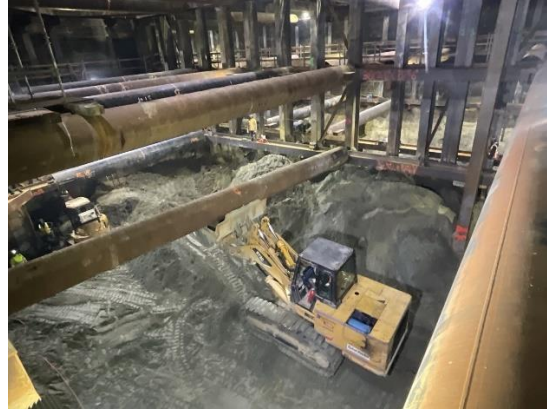
Century City Constellation Station Entrance excavation and strut installation
