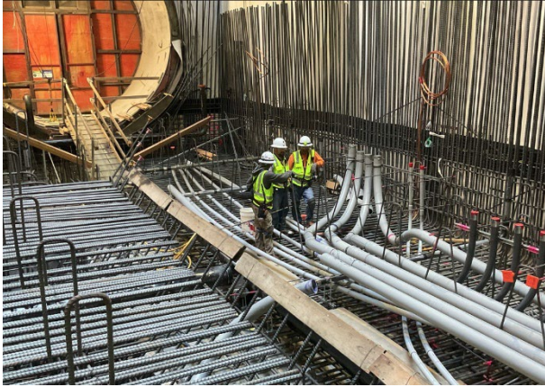
Conduit installation at CCCS Invert Slab
