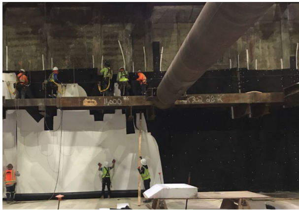
Waterproofing and Gas Venting System at the WRS Station
