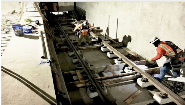
Track Installation at Wilshire/Western Interface Chamber
