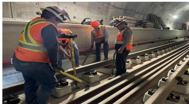
Reach 3 (BR) Track Installation
