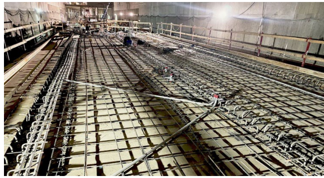
Platform Construction at Wilshire/La Cienega Station
