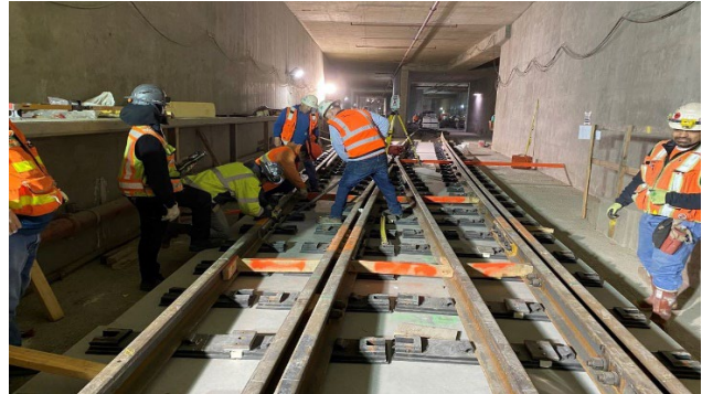
Crossover Construction at Wilshire/La Brea Station
